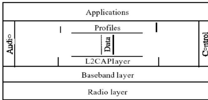
Figure 11 Bluetooth layers
