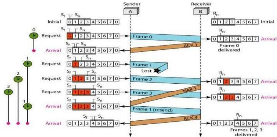
Figure 2.21 Flow diagram for Example 2.5
