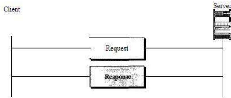
Figure 27.12 HTTP transaction
