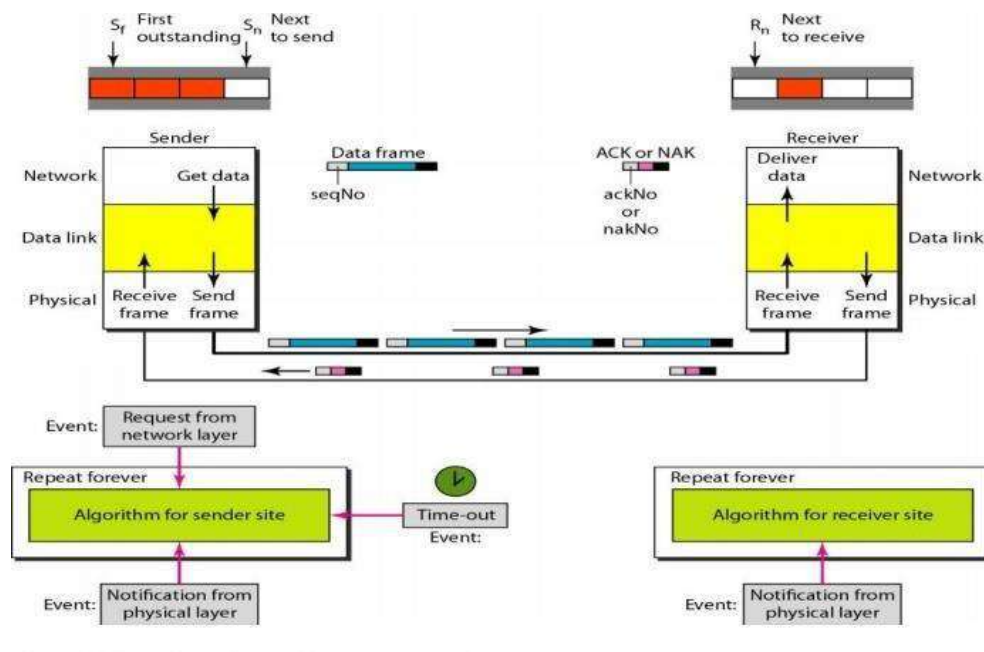
Figure 2.19 Design of Selective Repeat ARQ
