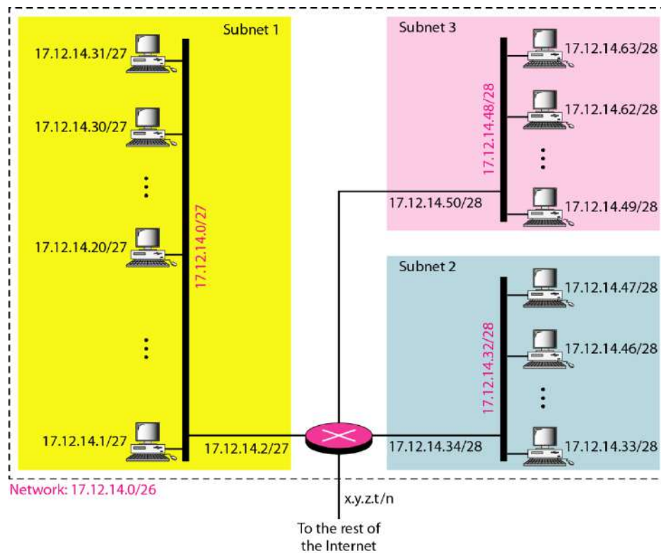
Figure 19.8 Three-level hierarchy in an IPv4 address
