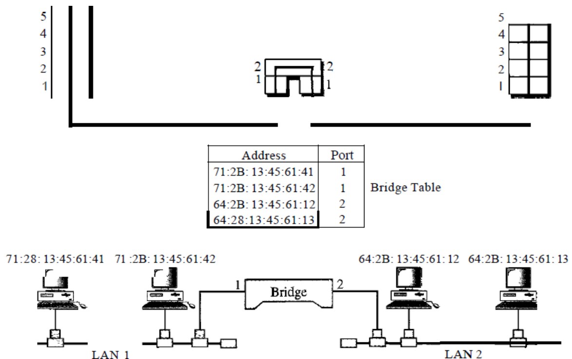
Figure. A bridge connecting two LANs
